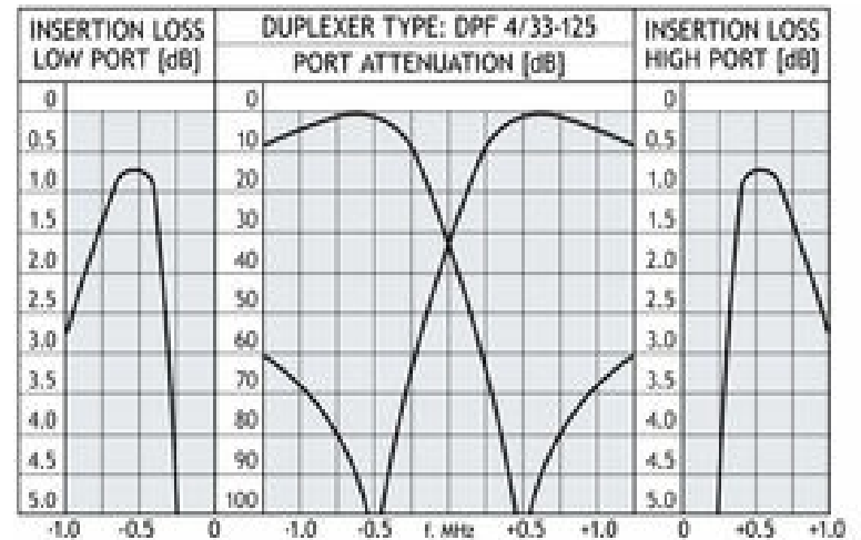
TYPICAL RESPONSE CURVES @ 1 MHZ DUPLEX SPACING
